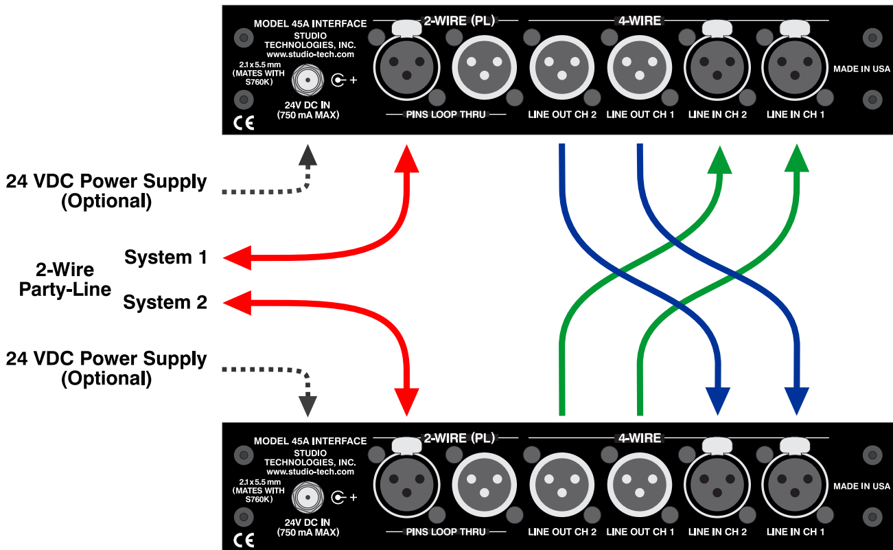
Figure 9. Two Model 45A units connected as a universal 2-wire-to-2-wire bridge
