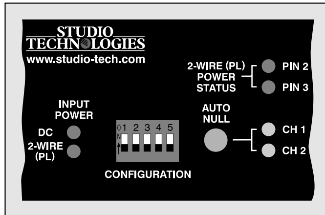
Figure 6. Details of front panel showing the five configuration DIP switches
