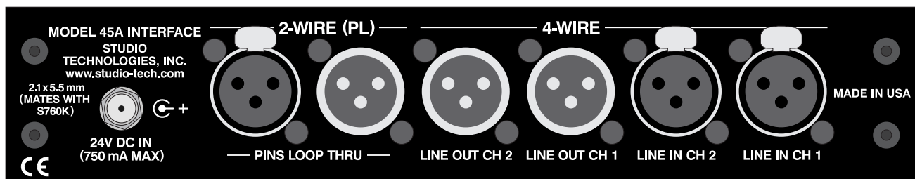
Figure 2. Model 45A back panel
